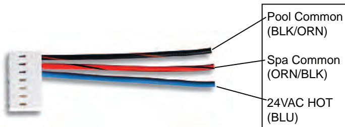
7-PIN Remote Wiring Connector
