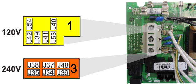
Voltage Selection Chart for 240V Conversion
