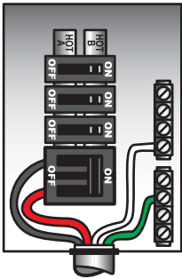
MAIN BREAKER PANEL
