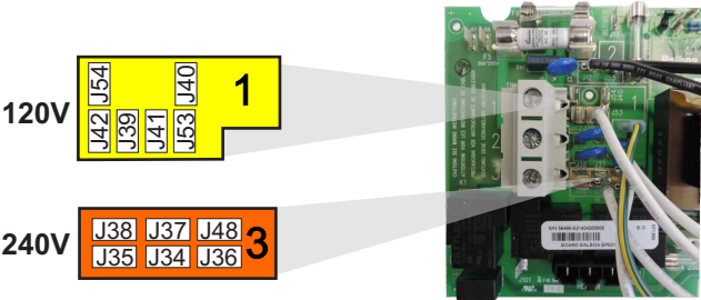
Voltage Selection Chart for 240V Conversion
