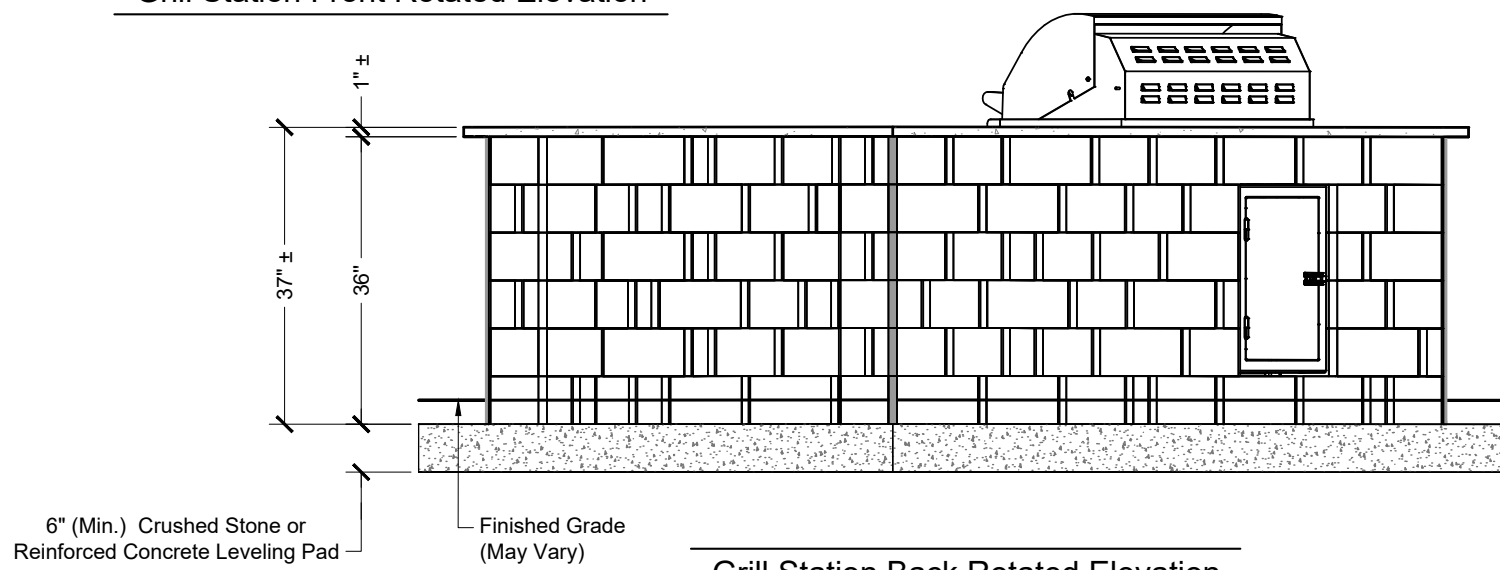
Grill Station Back Rotated Elevation
