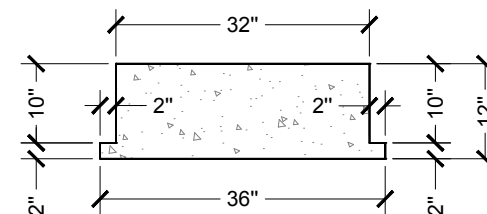
Grill Filler Piece Plan View Detail
