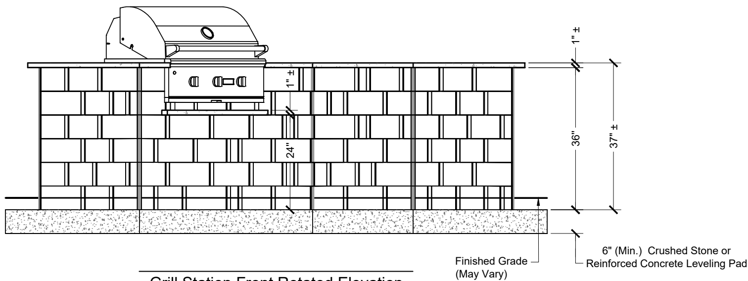
Grill Station Front Rotated Elevation
