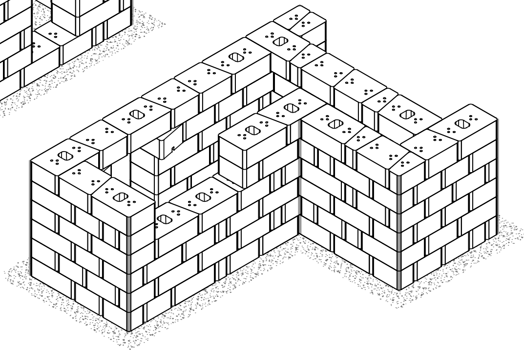
Grill Station Base Front Isometric
