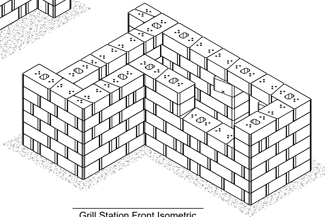
Grill Station Front Isometric
