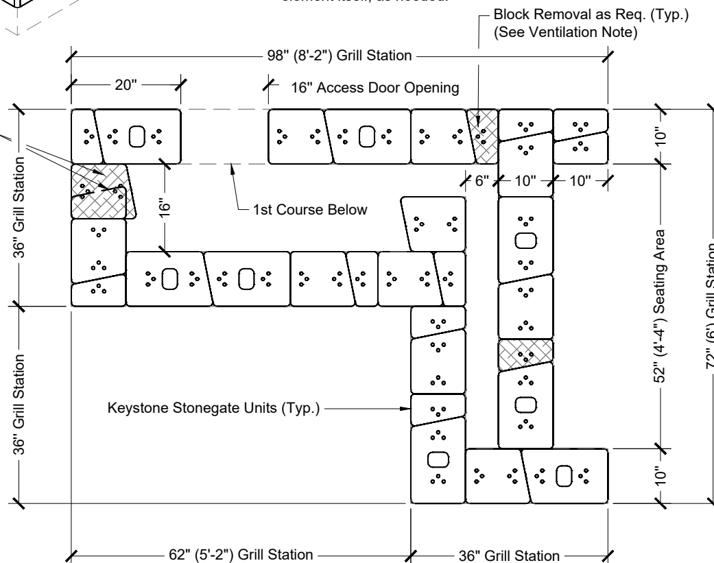
2nd Course Plan
