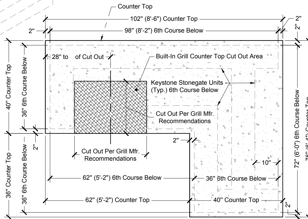
Grill Filler Piece Plan View Detail
