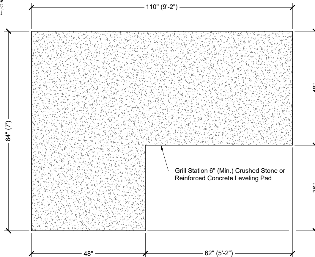
Foundation Plan
